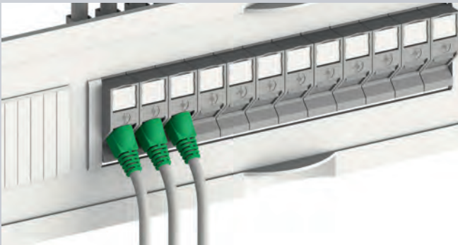
The height of the TS45 and cover inside the cabinet are optimally matched. The AMJ-S Module is installed so that the latch protection of the patch cord can be operated from above.
