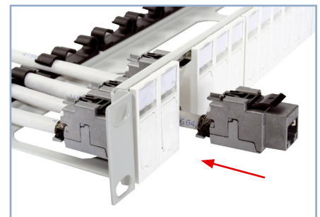
Installation from the front
